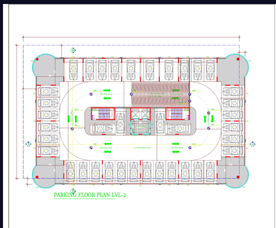
Parking - 2
