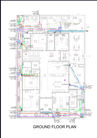
Ground · Water
