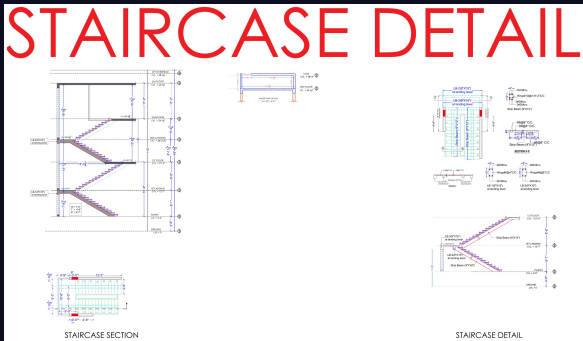
Staircase
