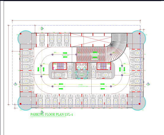
Parking · 1
